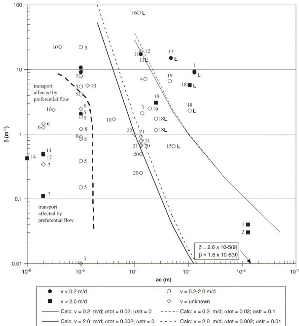
Fig. 9. Comparison of filter coefficients determined from field and laboratory studies and calculated filter coefficients. Parameters used to determine the calculated filter coefficients were a=0.02-0.002 , T=283 K, a_p=2 \mu\text{m} , and v=0.2-2.0 \text{ m d}^{-1} . See text for explanation. Parameters used to calculate filter coefficients were T=283 K, a_p=2 \mu\text{m} , \varepsilon=0.3 , H=6.5 \times 10^{-21} J; \rho_p=1050 \text{ kg m}^{-3} , \rho_{fl}=1000 \text{ kg m}^{-3} , \overline{u}=1.3 \times 10^{-3} \text{ kg s m}^{-1} ; area left of bold dashed line: transport of E. coli and thermotolerant coliforms is influenced by preferential flow. (1. Pang et al., 2003; 2. Sinton et al., 1997; 3. Caldwell, 1937; 4. Dyer, 1943-1945; 5. Smith et al., 1985; 6. Hagedorn et al., 1978; 7. Rahe et al., 1978; 8. McCoy and Hagedorn, 1980; 9. Sinton et al., 2000; 10. Butler et al., 1954; 11. Schaub and Sorber, 1977; 12. Bouwer et al., 1974a and Bouwer et al., 1974b; 13. Stevik et al., 1999; 14. McCoy and Hagedorn, 1979; 15. Powelson and Mills, 2001; 16. Goldshmid et al., 1973; 17. Viraraghavan, 1978; 18. Hijnen et al., 2004; 19. Ziebell et al., 1975; 20. Reneau and Pettry, 1975; 21. Reneau, 1978; 22. Schijven, 2001).
