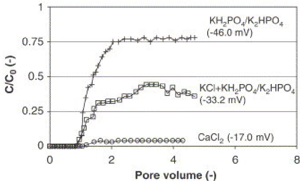
Fig. 5. Zeta potential values determined with the Helmholtz-Smoluchowski equation and breakthrough curves of E. coli ATCC 25922 suspended in various solutions ( \text{CaCl}_2 ; KCl and dilute phosphate buffered saline; phosphate buffered saline; C/C_0 data are from Powelson and Mills, 2001).
