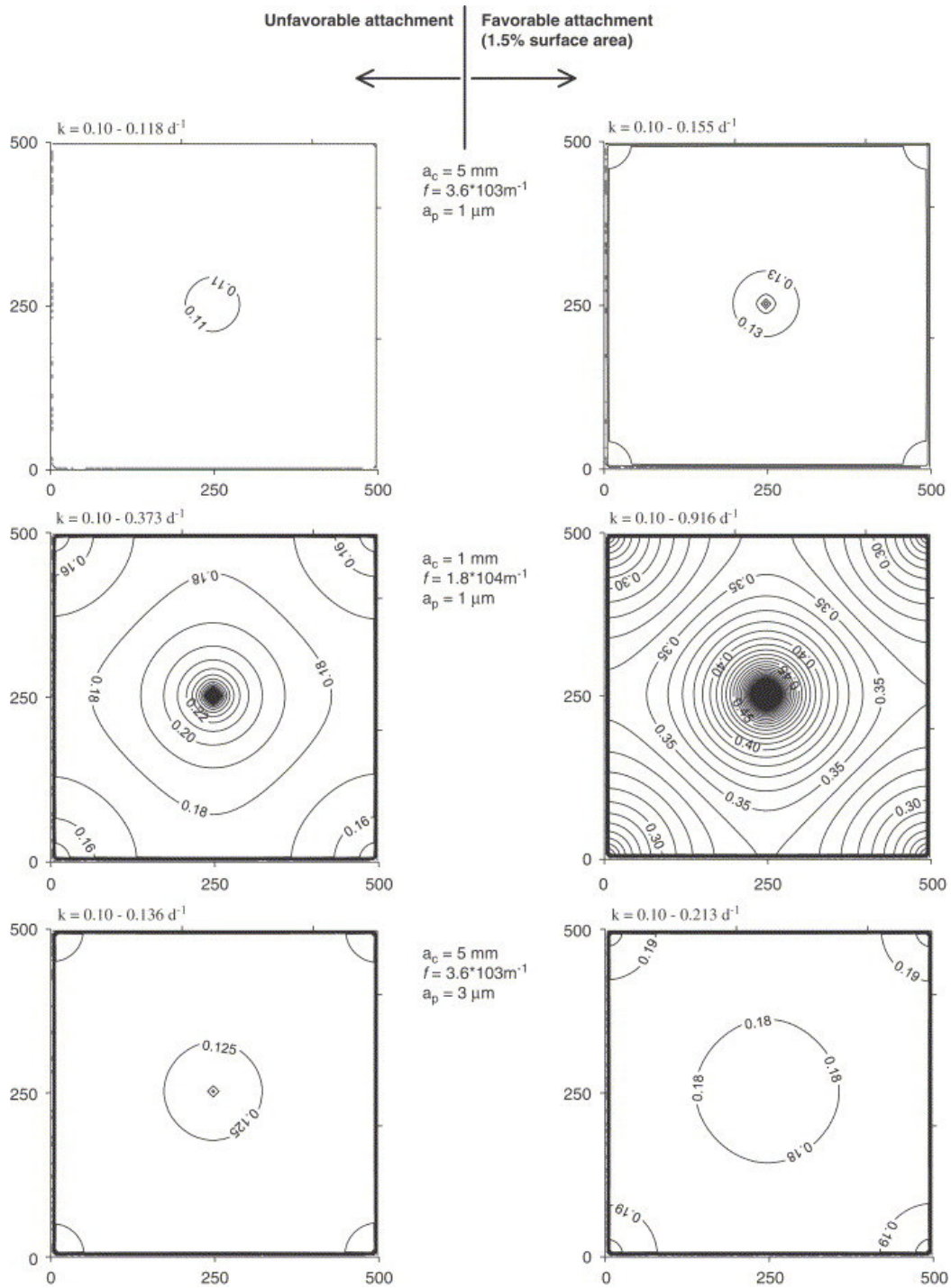
Fig. 12. Calculated total retention rate coefficient k_{total} (contour line interval: 0.01 \text{ d}^{-1} ). See text for explanation. Parameters used were a_{unfav}=0.007 , a_{fav}=1.00 , a_{str}=0.01 , k_i=0.1 \text{ d}^{-1} , T=283 \text{ K} , \epsilon=0.25 , H=6.5 \times 10^{-21} \text{ J} ; \rho_p=1050 \text{ kg m}^{-3} , \rho_{fl}=1000 \text{ kg m}^{-3} , \omega=1.3 \times 10^{-3} \text{ kg s m}^{-1} ; left-hand graphs: \lambda=0 , right-hand graphs: \lambda=0.015 .
