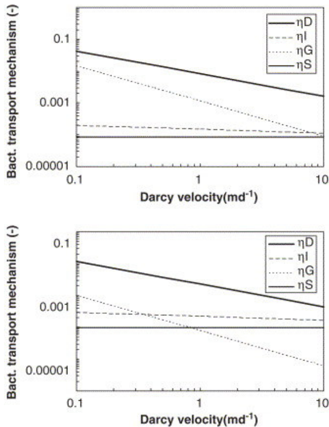
Fig 2. Magnitude of the single bacterial transport mechanisms as a function of Darcy flow velocity. Upper graph: a_c=1 mm; lower graph: a_c=0.02 mm. Other parameters (for both graphs): T=283 K, a_p=1 \mu m, \epsilon=0.35 , H=6.5 \times 10^{-21} J; \rho_p=1050 kg m -3 , \rho_{fl}=1000 kg m -3 , \omega=1.3 \times 10^{-3} kg s m -1 .
