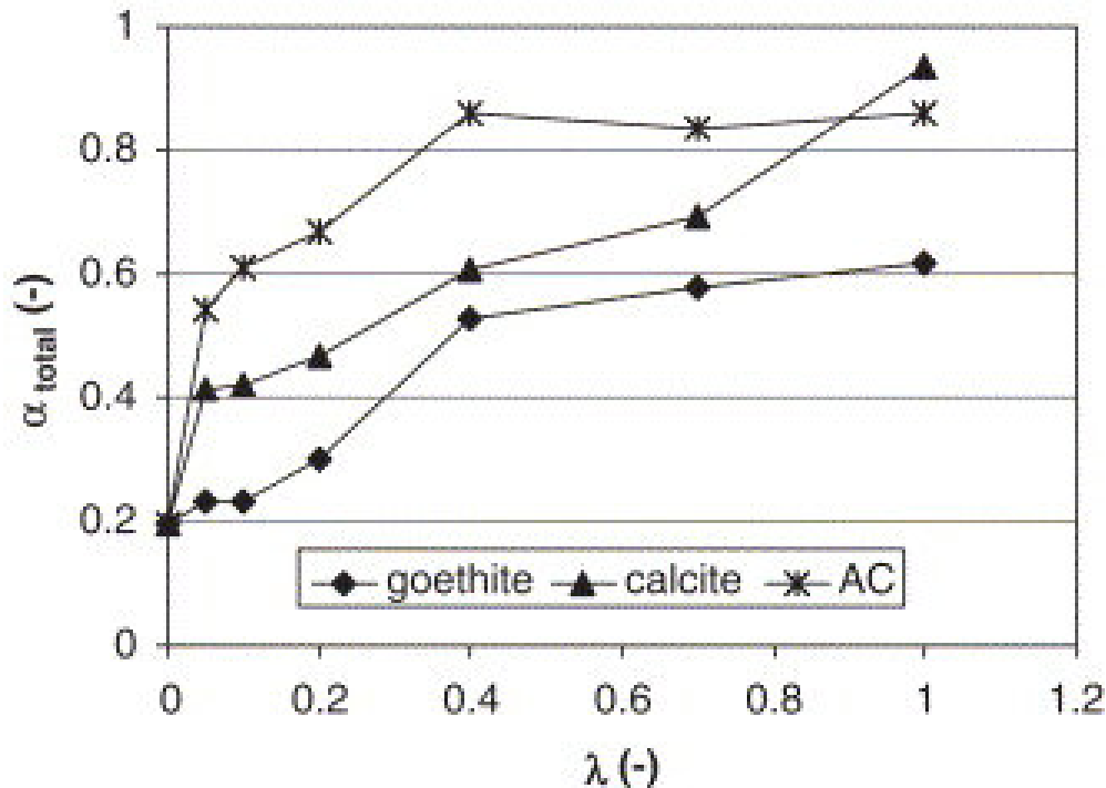
Fig. 8. Relation between calculated total sticking efficiency ( \alpha_{total} ) and geochemical heterogeneity parameter ( \lambda ) for experiments carried out with quartz sand and goethite coated sand, quartz sand and calcite grains, and quartz sand and granular activated carbon (from: Foppen and Schijven, 2005). Fractions of goethite, calcite, and granular activated carbon varied from 5% to 100%.
