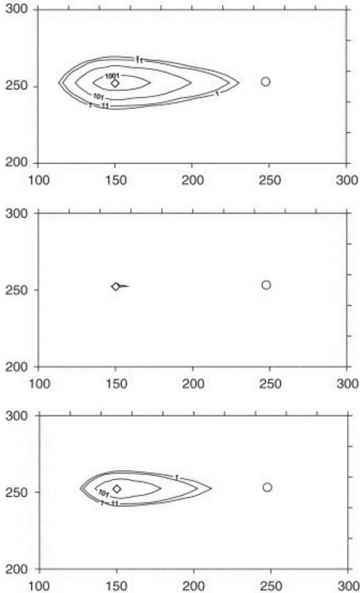
Fig. 13. Distribution of E. coli concentration (in \text{cells}(\text{mL})^{-1} ) midway in layer 2 at a depth of 12.5 m after 100 days of infiltration. The abstraction well is given as a circle and the recharge well is a diamond (the recharge well is located in the middle of layer 1 at a depth of 2.5 m). Retention rate coefficients used are given in Fig. 12 (right-hand part) for the case of favorable attachment.
