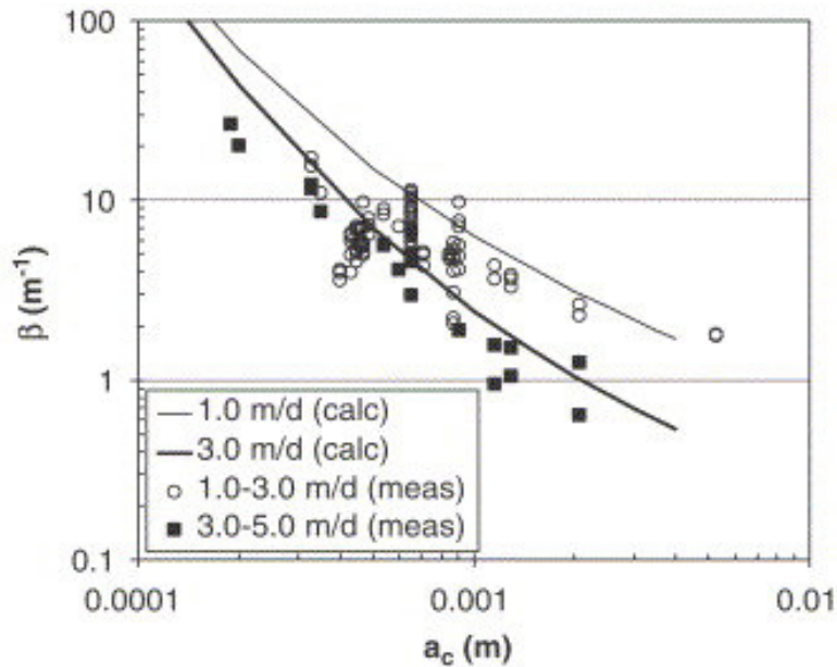
Fig. 4. Comparison of measured and calculated filter coefficients as a function of the median of the grain size number distribution (m) and Darcy flow velocity ( \text{m d}^{-1} ). The calculated filter coefficient was determined with the SCCE according to the TE correction equation (Tufenkji and Elimelech, 2004a) and a collision efficiency, \alpha=0.43 .
