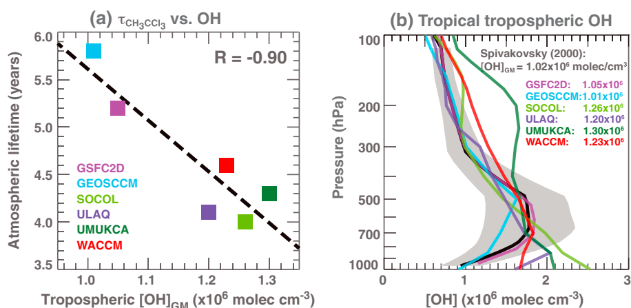
Figure 2. (a) Modeled steady state atmospheric lifetimes (years) from the TS2000 simulation for \text{CH}_3\text{CCl}_3 versus mass-weighted tropospheric OH abundance. (b) Comparison of tropical ( 30^\circ\text{S} – 30^\circ\text{N} ) annual mean OH profiles from Spivakovsky et al. (2000) (thick black line with gray shading indicates 1\sigma spatial and temporal variance in that model) and the models. The global mean OH abundances from Spivakovsky et al. (2000) and those derived from the models ( [\text{OH}]_{\text{GM}} ; molecules \text{cm}^{-3} ) are given in the legend. All CCM results are 30 year annual average from the 2000 time-slice simulations.
