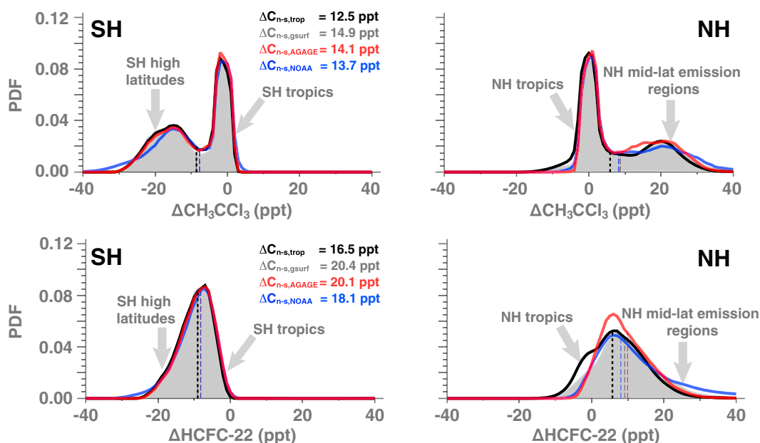
Figure 9. The model probability distribution function of the (left) SH and (right) NH detrended mixing ratio anomalies (with respect to global mean values) for \text{CH}_3\text{CCl}_3 and HCFC-22 during 1980–2014. \Delta C_{n-s} calculated using all global surface grids ( \Delta C_{n-s,gsurf} ; gray shading for distribution probability and thin gray dashed lines for area-weighted hemispheric mean anomaly) differ from those calculated using the modeled values sampled at the AGAGE stations (thick red lines for distribution probability and red dashed lines for hemispheric mean) and the NOAA-GMD stations (thick blue lines for distribution probability and blue dashed lines for hemispheric mean). Station-based values are interpolated to all latitudes, from 90°S to 90°N, for full global representation. The modeled distribution probability (thick black lines), hemispheric means (black dashed lines), and \Delta C_{n-s,trop} calculated using all grid cell results below 500 hPa are also shown.
