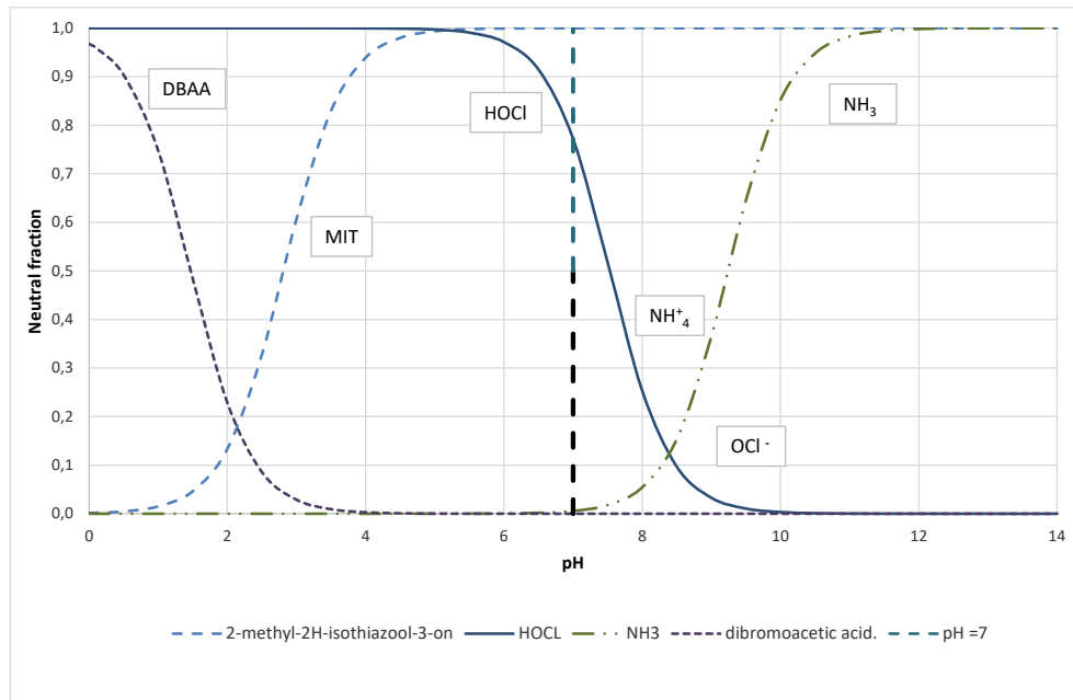
Figure 6 Speciation (neutral fraction) of acids and bases as a function of the pH of the solution.
